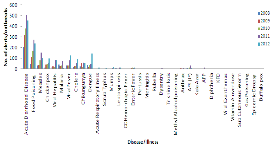
Comparison of cumulative number of disease alerts/outbreaks reported till the 46th week of 2008, 2009, 2010, 2011 & 2012
